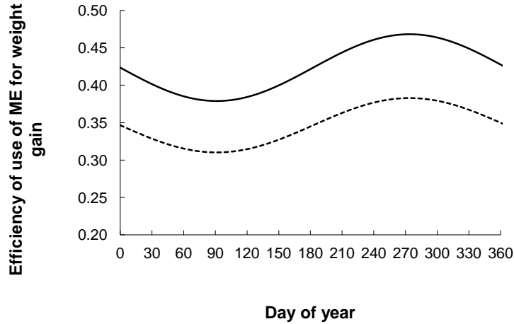
Fig. 7. The efficiency of the use of metabolizable energy for weight gain, in relation to herbage metabolizability, M/D, and time of year, for a pasture diet containing 30% legume and at a latitude of 35°S; upper line, M/D = 11; lower line, M/D = 9.
