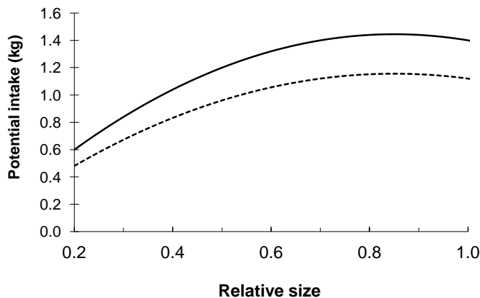
Fig. 2. Potential daily intake of dry matter by a sheep with a standard reference weight of 50 kg (solid line) or 40 kg (dashed line), in relation to its relative size, for an animal that is not lactating and has a relative condition \leq 1.0 .
