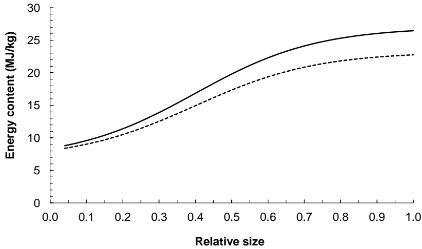
Fig.13. Energy content of empty weight gain at a feeding level of twice maintenance, in relation to the relative size of the animal: upper line, sheep and standard cattle; lower line, lean cattle types.
